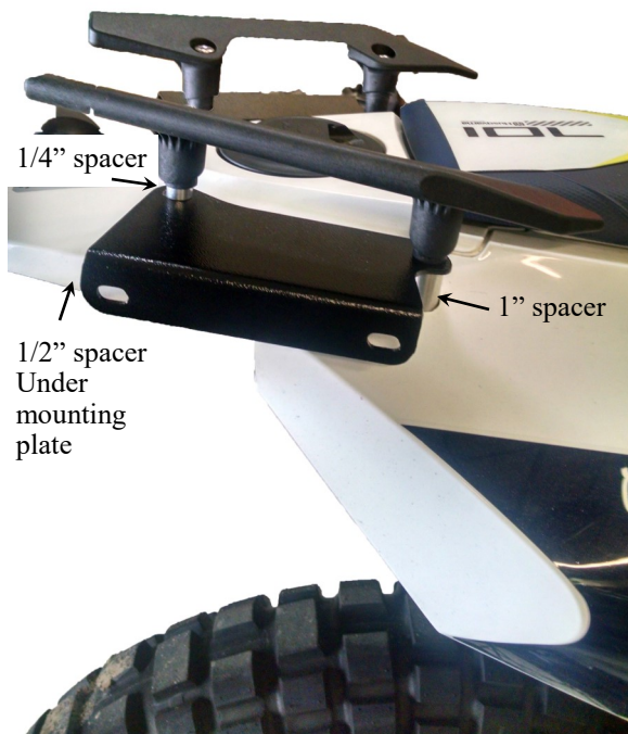
Figure 2 The grab handles mounted on top of SU mounting plate.
