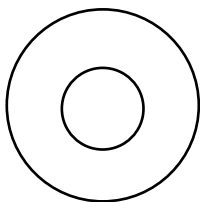
OD3/4, ID .319, L 3/4 Spacer (Countersunk on top)
